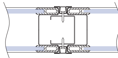
Double glazed mullion
