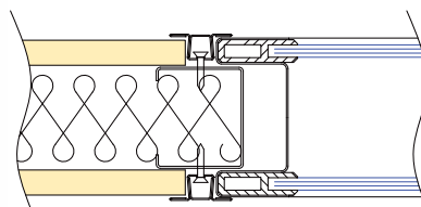
Double glazed to solid mullion
